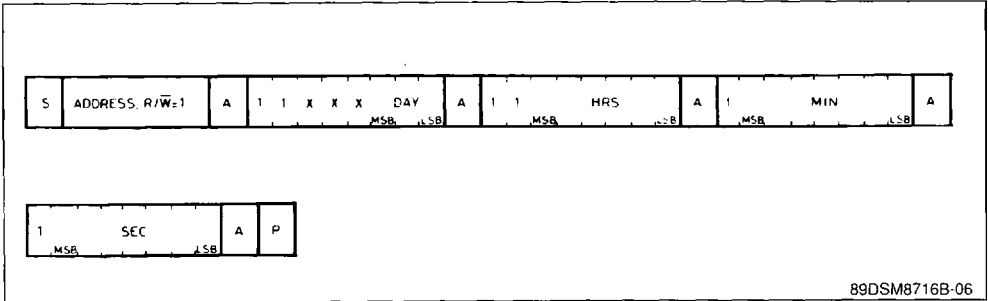
Figure 3b : Data Format for One Cycle Address/-write (with day of week indication).
