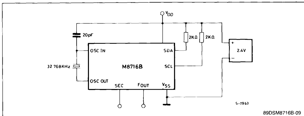
Figure 5 : Test Circuit.
