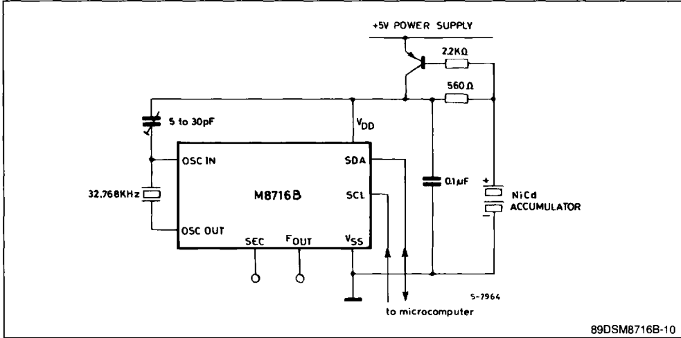
Figure 6 : Typical Application.
